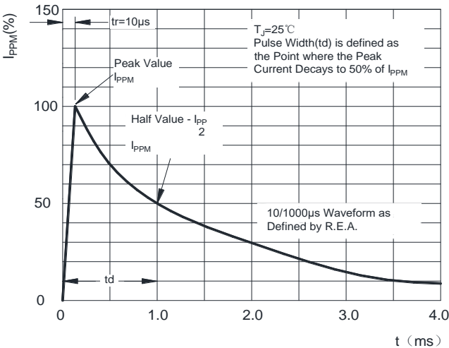
FIG3: Pulse Waveform
